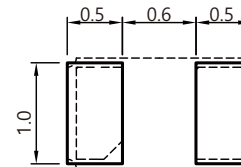
Land Pattern
