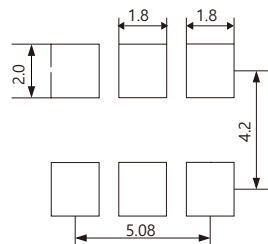
Land Pattern
