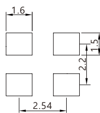
Land Pattern
